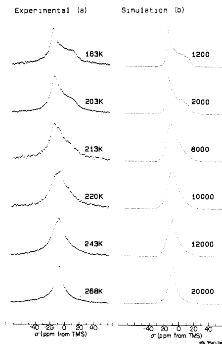
Figure 2. Experimental (a) and simulated (b) ^1\text{H} spectra of proton-doped (0.5%) hexagonal \text{D}_2\text{O} . Each simulation is labeled with the rate \Omega = 1/\tau_c .
